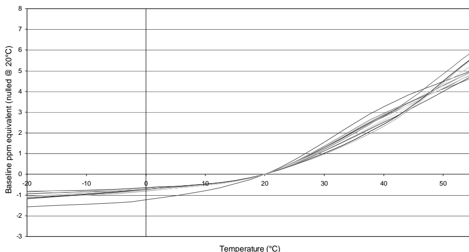
4ETO Ethylene Oxide CiTiceL - Baseline vs Temperature
