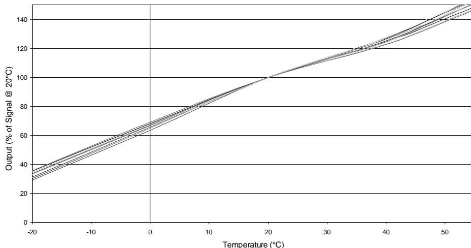
4ETO Ethylene Oxide CiTiceL - Output vs Temperature
